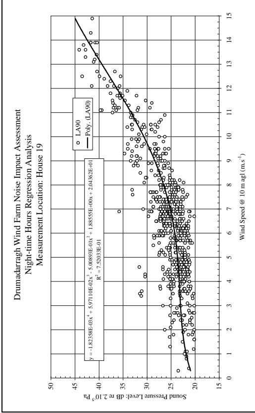
Regression Figure 2
