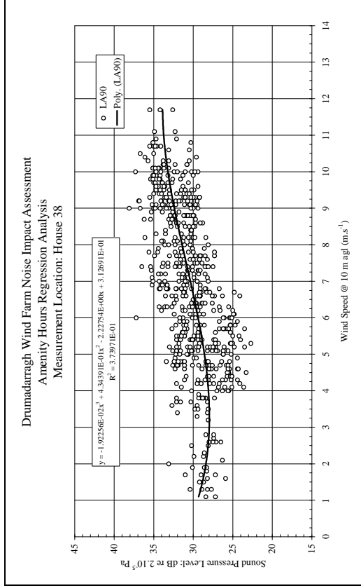
Regression Figure 3
